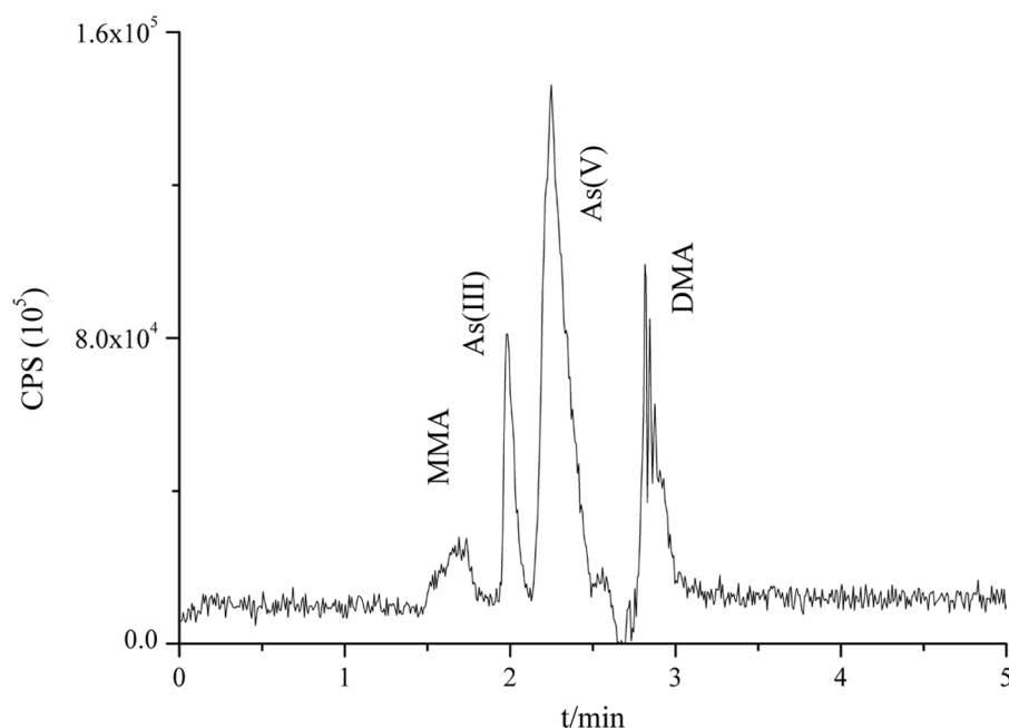
FIGURE 3 Electropherograms of urine containing arsenite (As (III)), arsenate (As (V)), monomethyl arsonic acid (MMA), and dimethyl arsinic acid (DMA). With addition of 200 mg/L at final concentration of MMA (a) and As(V).
