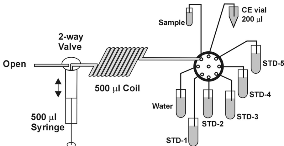
FIGURE 1 Scheme of the SIA system employed. The syringe pump of 500 \mu L, the As standard solutions, the holding coil and the small vials 200 \mu L.
